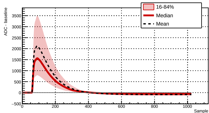
Run 043380 - Channel 2081 - 6486 waveforms
