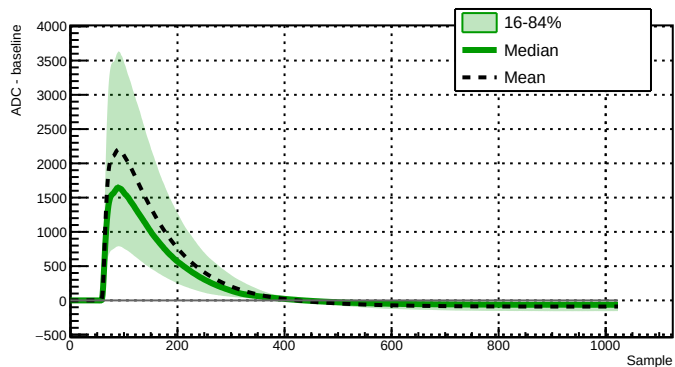
Run 043380 - Channel 2080 - 5290 waveforms
