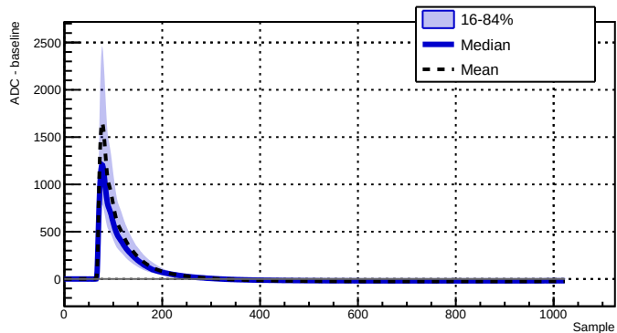
Run 043380 - Channel 2070 - 2239 waveforms
