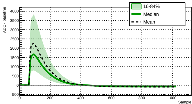
Run 043381 - Channel 2080 - 5333 waveforms
