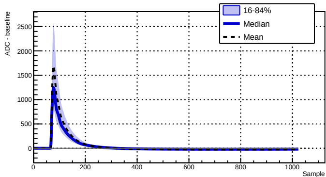
Run 043381 - Channel 2070 - 2233 waveforms
