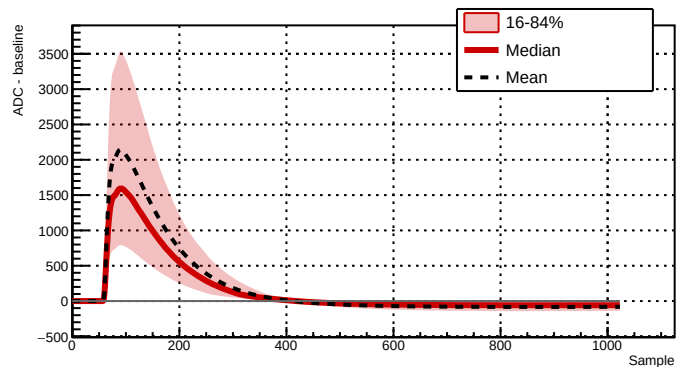
Run 043381 - Channel 2081 - 6547 waveforms
