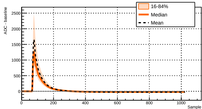
Run 043381 - Channel 2071 - 2290 waveforms
