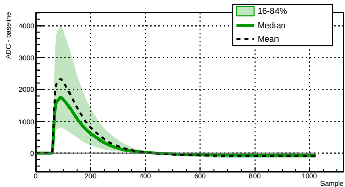
Run 043384 - Channel 2080 - 5652 waveforms
