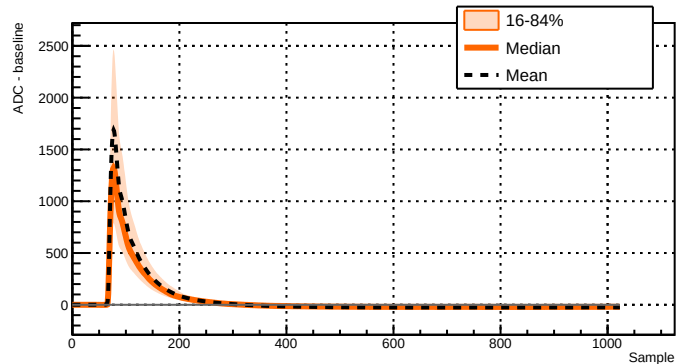
Run 043384 - Channel 2071 - 2589 waveforms
