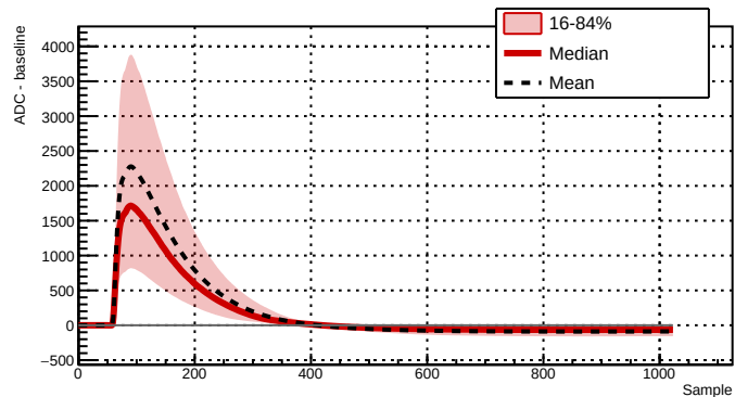
Run 043384 - Channel 2081 - 6954 waveforms
