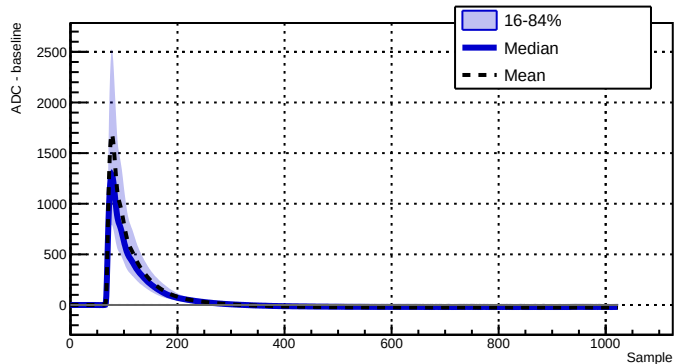
Run 043384 - Channel 2070 - 2438 waveforms
