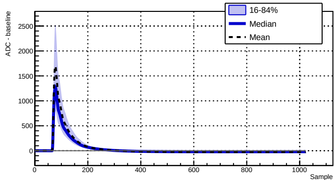
Run 043386 - Channel 2070 - 2303 waveforms
