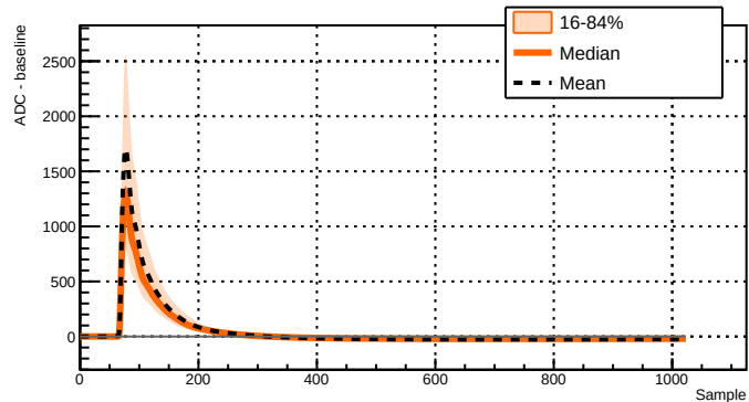
Run 043386 - Channel 2071 - 2400 waveforms
