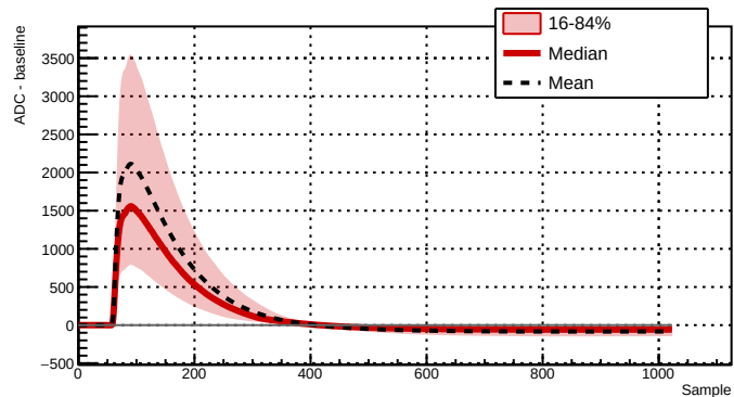
Run 043386 - Channel 2081 - 6503 waveforms
