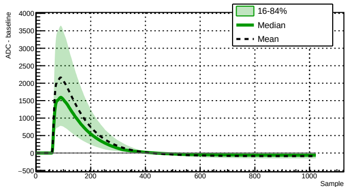
Run 043386 - Channel 2080 - 5223 waveforms
