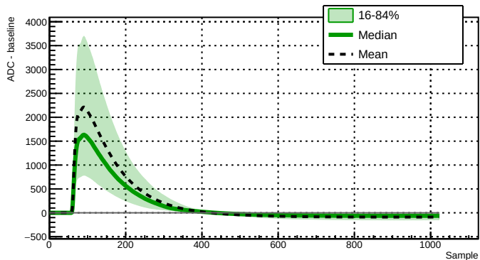
Run 043387 - Channel 2080 - 5220 waveforms
