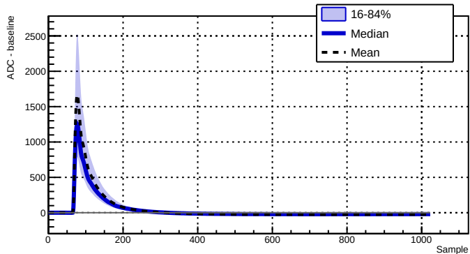
Run 043387 - Channel 2070 - 2198 waveforms
