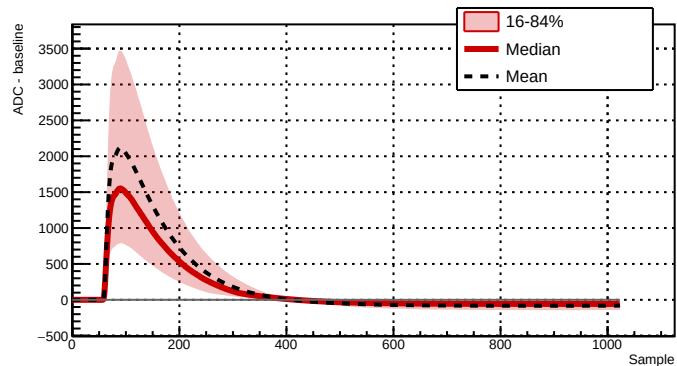
Run 043387 - Channel 2081 - 6459 waveforms
