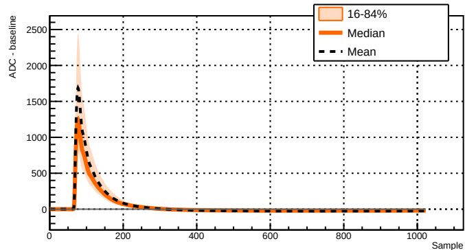
Run 043387 - Channel 2071 - 2252 waveforms
