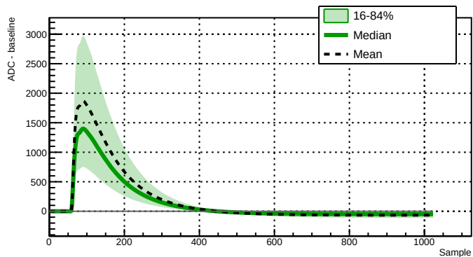
Run 039500 - Channel 2080 - 28366 waveforms
