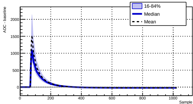
Run 039500 - Channel 2070 - 7854 waveforms
