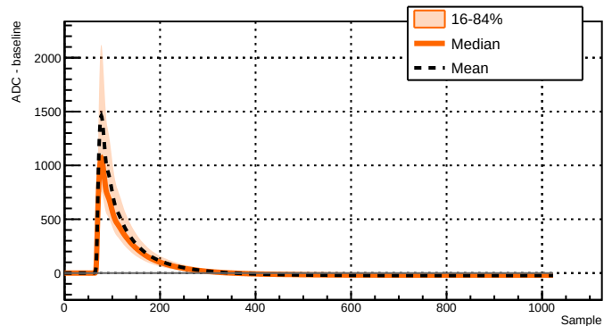
Run 039500 - Channel 2071 - 7635 waveforms
