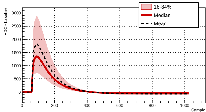
Run 039500 - Channel 2081 - 28202 waveforms
