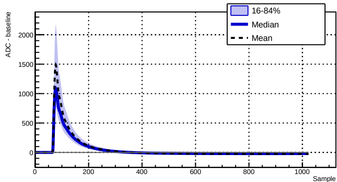
Run 039501 - Channel 2070 - 8096 waveforms
