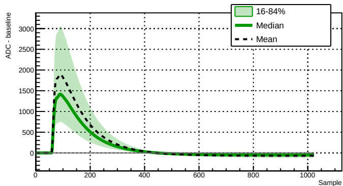
Run 039501 - Channel 2080 - 29318 waveforms
