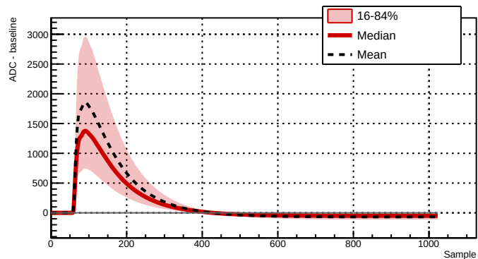
Run 039501 - Channel 2081 - 29094 waveforms
