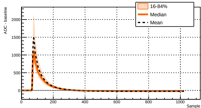
Run 039501 - Channel 2071 - 7918 waveforms
