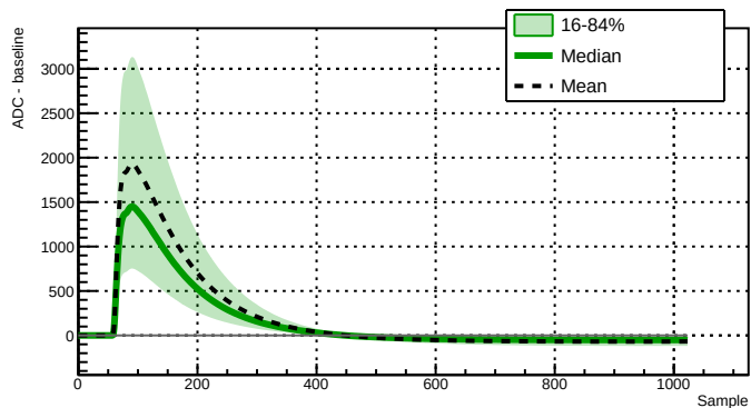
Run 039502 - Channel 2080 - 30306 waveforms
