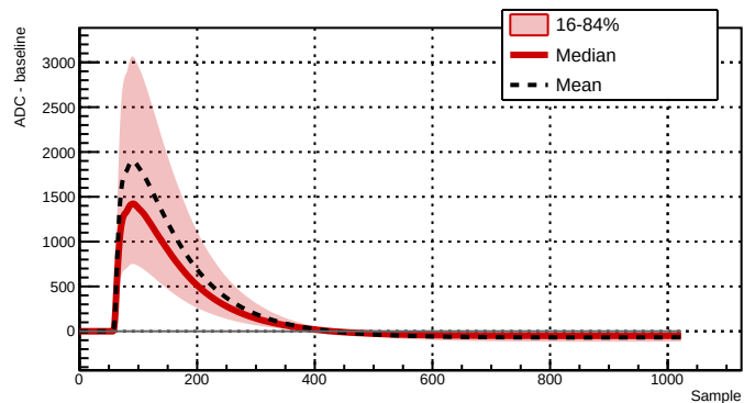
Run 039502 - Channel 2081 - 29934 waveforms
