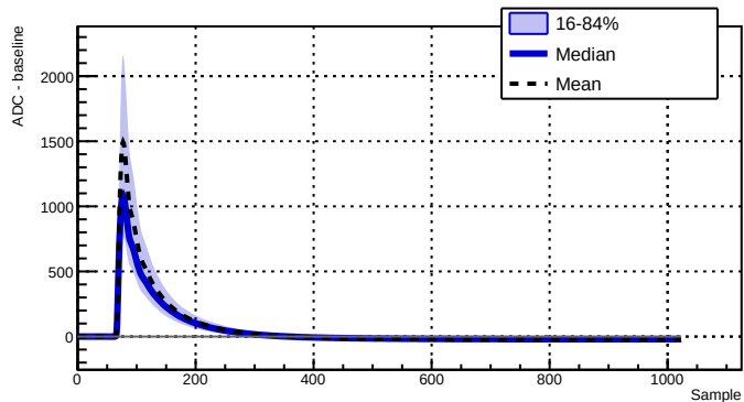
Run 039502 - Channel 2070 - 8514 waveforms
