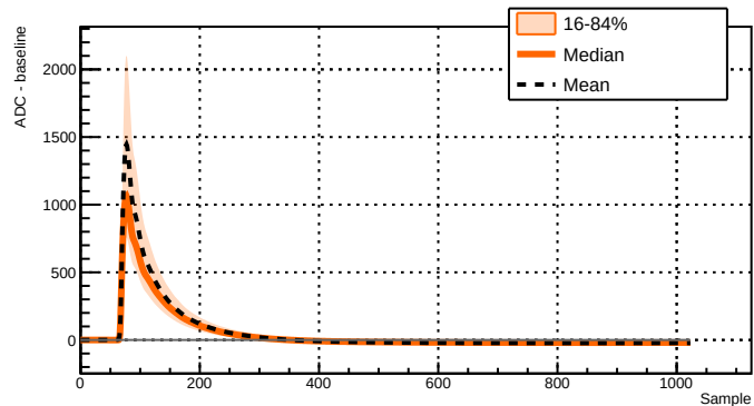
Run 039503 - Channel 2071 - 8989 waveforms
