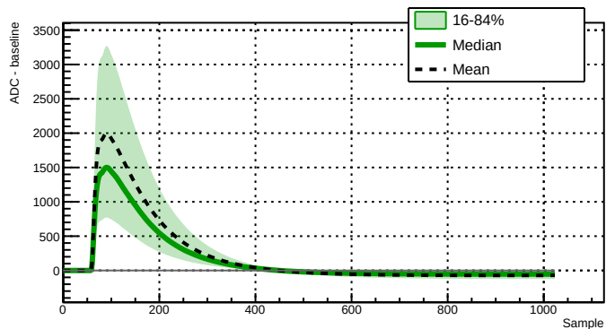
Run 039503 - Channel 2080 - 31688 waveforms
