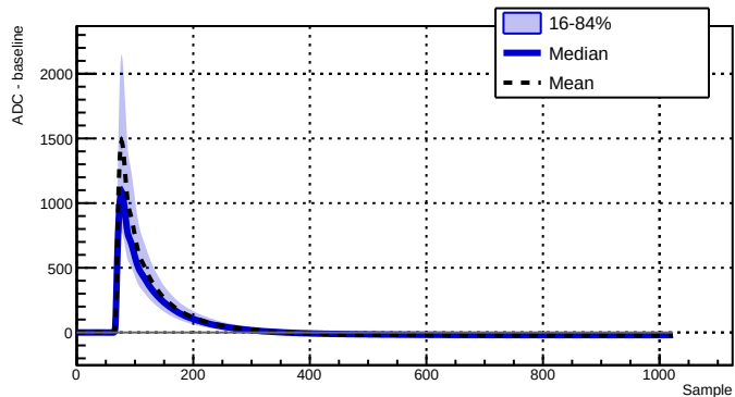
Run 039503 - Channel 2070 - 9047 waveforms
