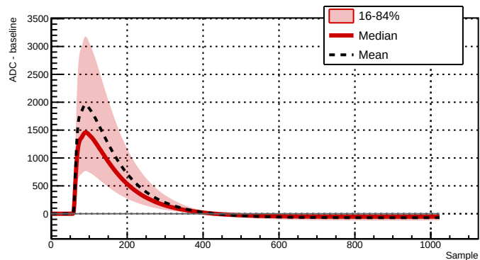
Run 039503 - Channel 2081 - 31461 waveforms
