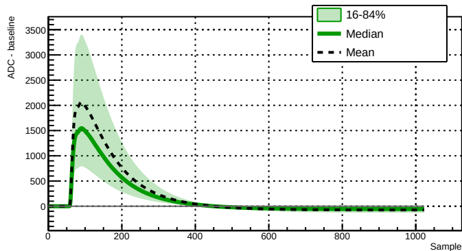
Run 039504 - Channel 2080 - 32478 waveforms
