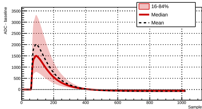
Run 039504 - Channel 2081 - 32275 waveforms
