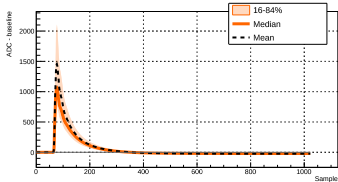
Run 039504 - Channel 2071 - 9375 waveforms
