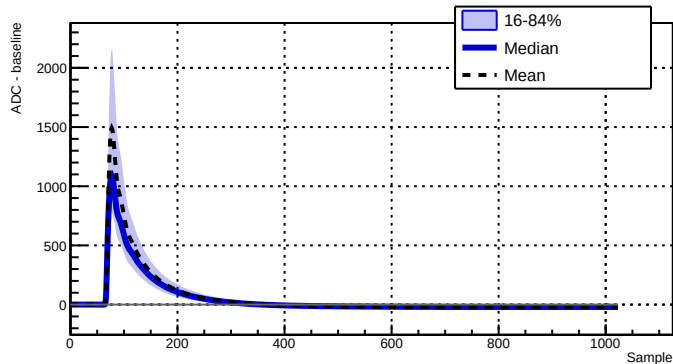
Run 039504 - Channel 2070 - 9343 waveforms
