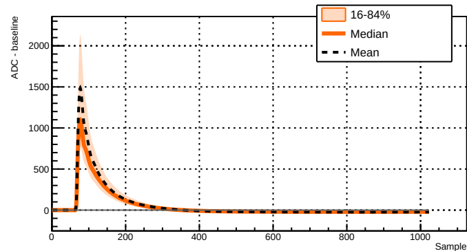
Run 039506 - Channel 2071 - 9974 waveforms
