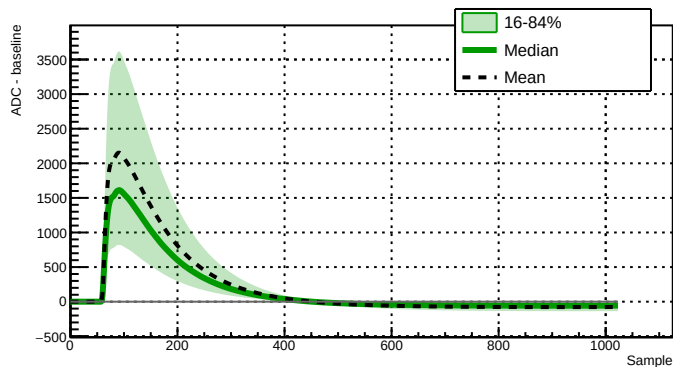
Run 039506 - Channel 2080 - 34052 waveforms
