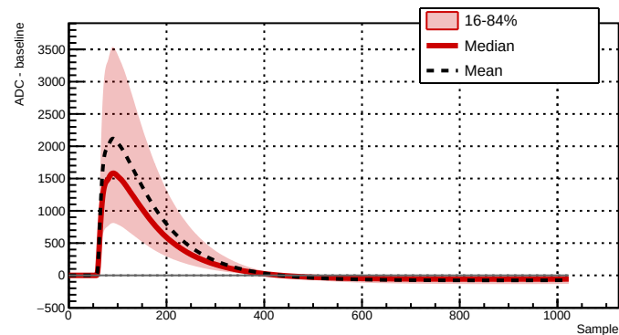
Run 039506 - Channel 2081 - 33719 waveforms
