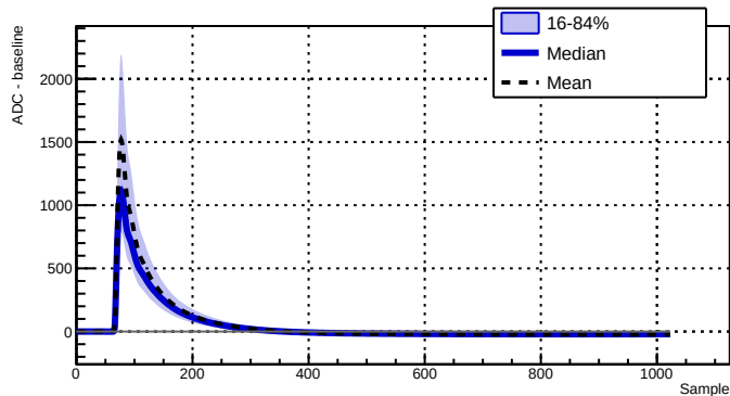
Run 039506 - Channel 2070 - 10020 waveforms
