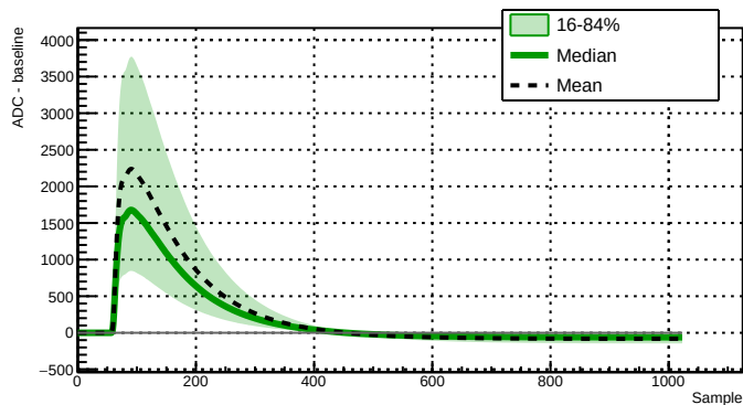
Run 039507 - Channel 2080 - 35929 waveforms
