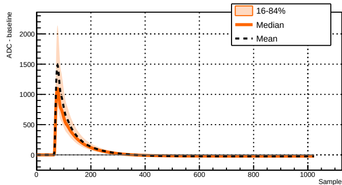
Run 039507 - Channel 2071 - 10608 waveforms
