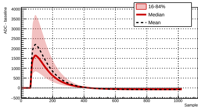
Run 039507 - Channel 2081 - 35559 waveforms
