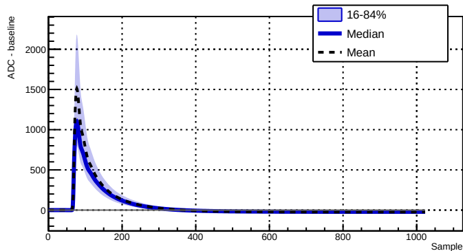
Run 039507 - Channel 2070 - 10726 waveforms
