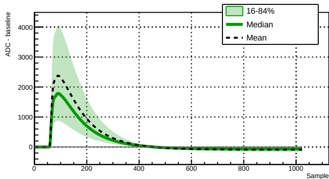
Run 039508 - Channel 2080 - 37048 waveforms
