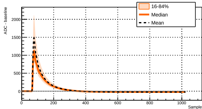
Run 039508 - Channel 2071 - 11551 waveforms
