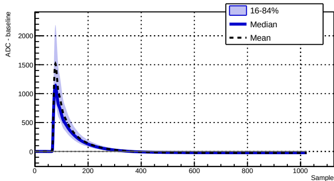
Run 039508 - Channel 2070 - 11555 waveforms
