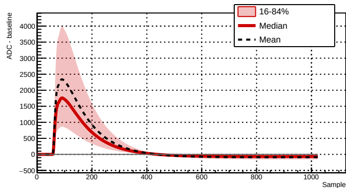
Run 039508 - Channel 2081 - 36823 waveforms
