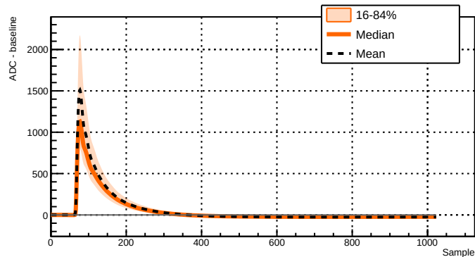
Run 039512 - Channel 2071 - 11685 waveforms
