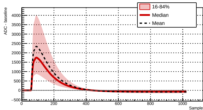
Run 039512 - Channel 2081 - 36975 waveforms
