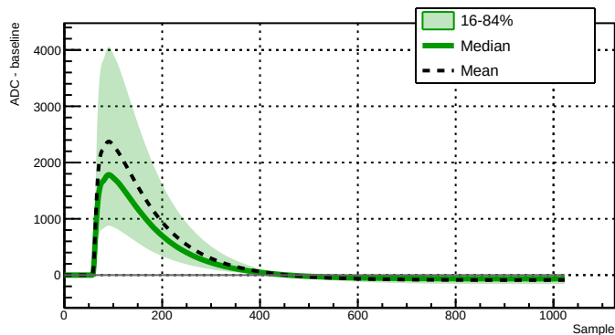
Run 039512 - Channel 2080 - 37206 waveforms
