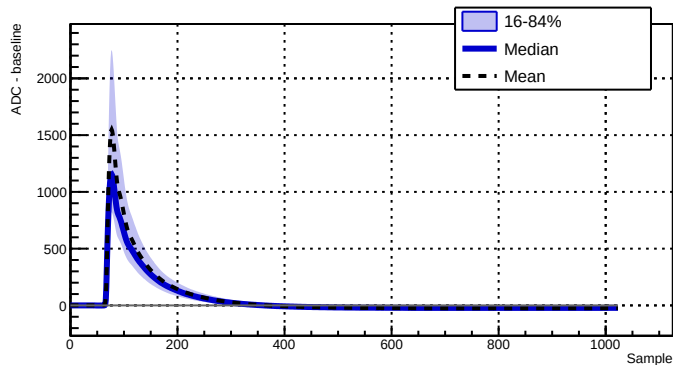
Run 039512 - Channel 2070 - 11581 waveforms
