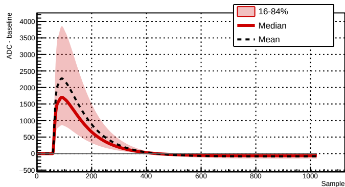
Run 039514 - Channel 2081 - 35609 waveforms
