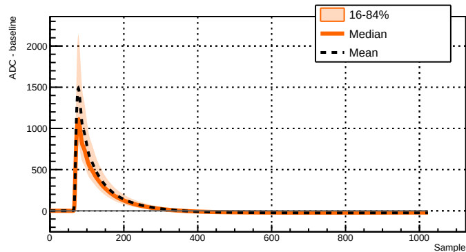
Run 039514 - Channel 2071 - 10968 waveforms
