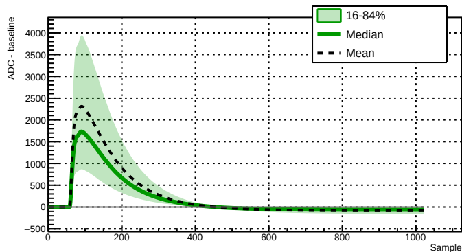
Run 039514 - Channel 2080 - 35936 waveforms
