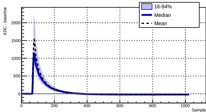
Run 039514 - Channel 2070 - 10986 waveforms
