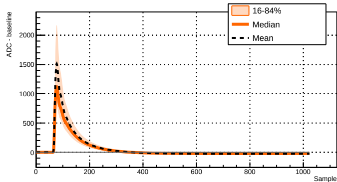
Run 039515 - Channel 2071 - 10408 waveforms
