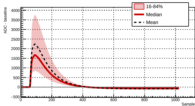
Run 039515 - Channel 2081 - 33999 waveforms
