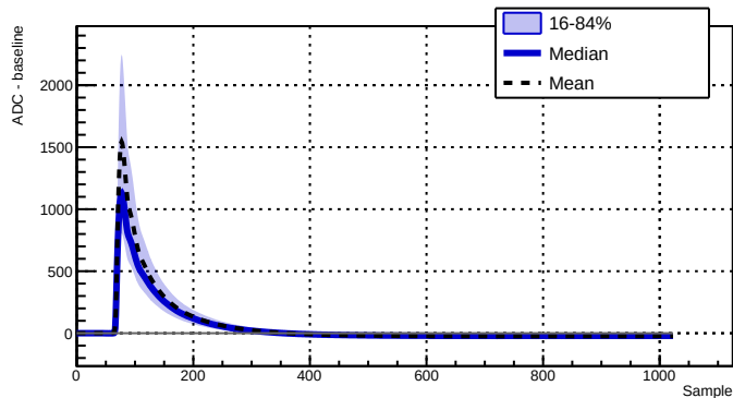
Run 039515 - Channel 2070 - 10523 waveforms
