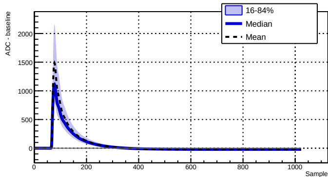
Run 039516 - Channel 2070 - 10151 waveforms
