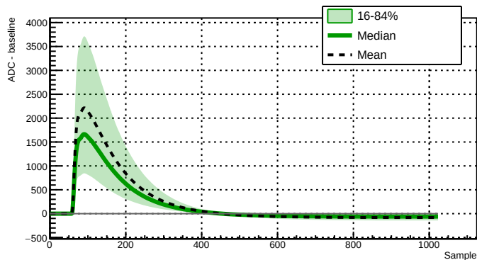
Run 039516 - Channel 2080 - 33362 waveforms
