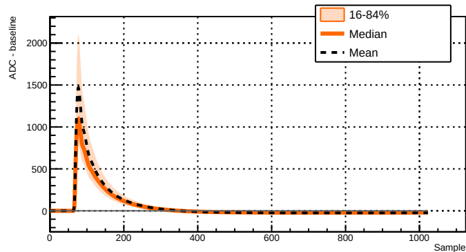
Run 039516 - Channel 2071 - 10059 waveforms
