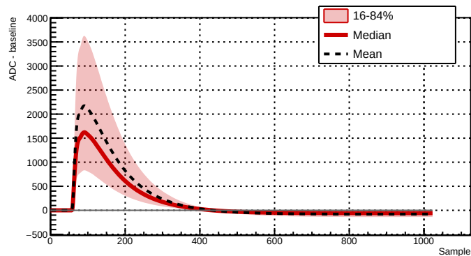
Run 039516 - Channel 2081 - 33160 waveforms
