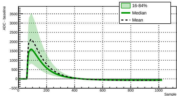
Run 039518 - Channel 2080 - 32734 waveforms
