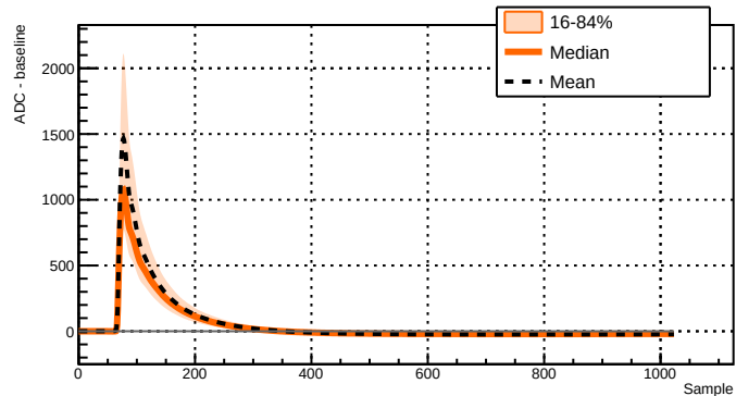
Run 039518 - Channel 2071 - 9627 waveforms
