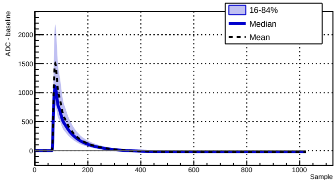
Run 039518 - Channel 2070 - 9539 waveforms
