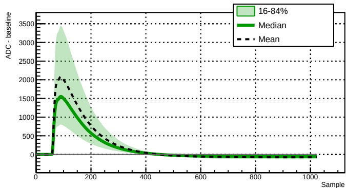
Run 039519 - Channel 2080 - 32310 waveforms
