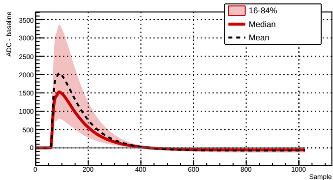
Run 039519 - Channel 2081 - 32080 waveforms
