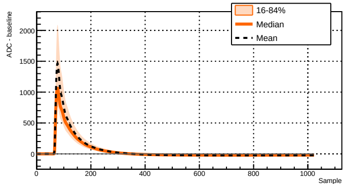
Run 039519 - Channel 2071 - 9330 waveforms
