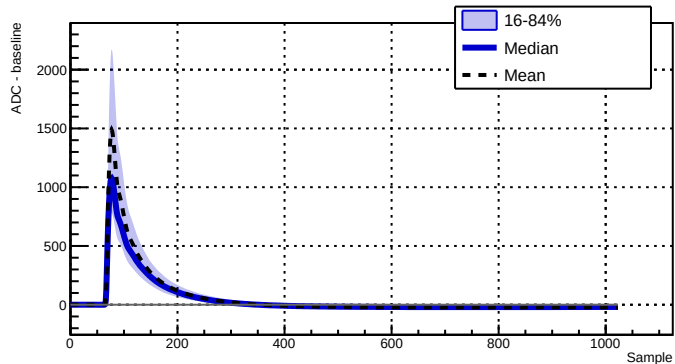
Run 039519 - Channel 2070 - 9429 waveforms
