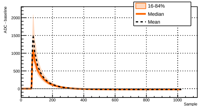
Run 039521 - Channel 2071 - 8956 waveforms
