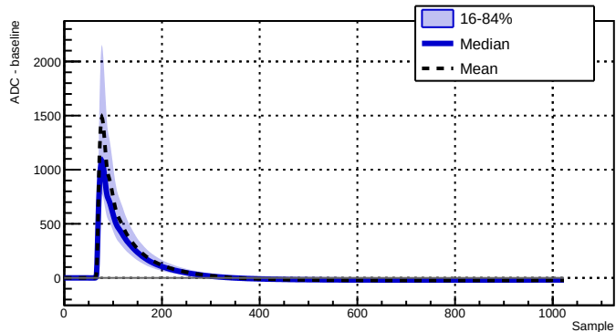
Run 039521 - Channel 2070 - 9036 waveforms
