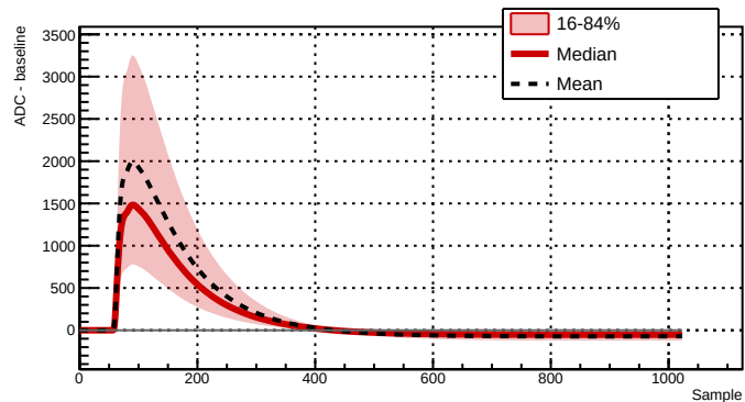
Run 039521 - Channel 2081 - 30964 waveforms
