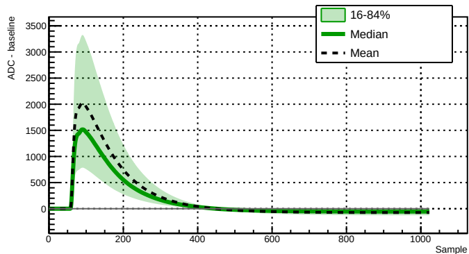
Run 039521 - Channel 2080 - 31285 waveforms
