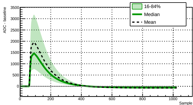
Run 039523 - Channel 2080 - 30261 waveforms
