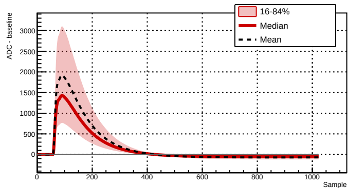
Run 039523 - Channel 2081 - 30050 waveforms
