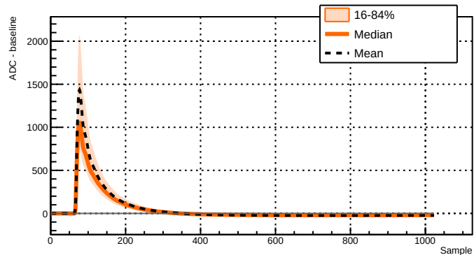
Run 039523 - Channel 2071 - 8539 waveforms
