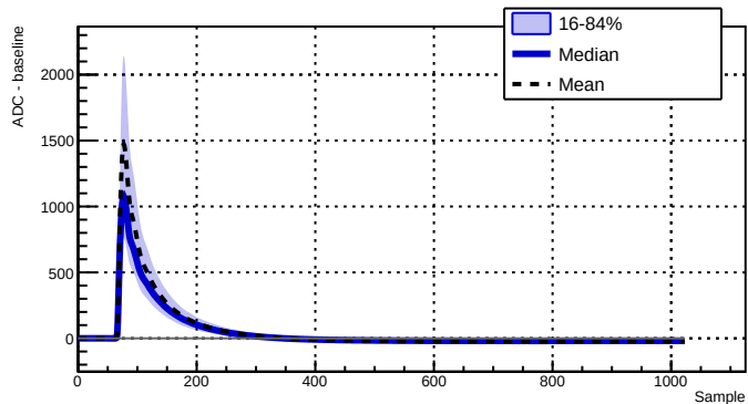
Run 039523 - Channel 2070 - 8572 waveforms
