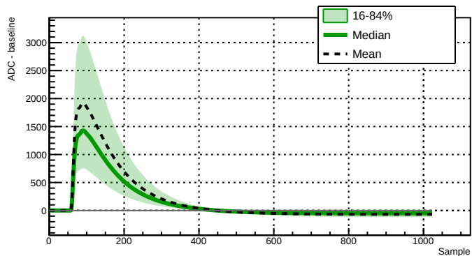
Run 039526 - Channel 2080 - 29292 waveforms
