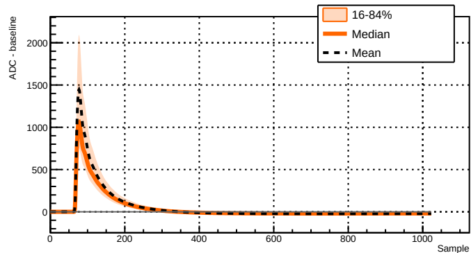
Run 039526 - Channel 2071 - 8088 waveforms
