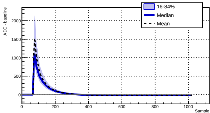
Run 039526 - Channel 2070 - 8134 waveforms
