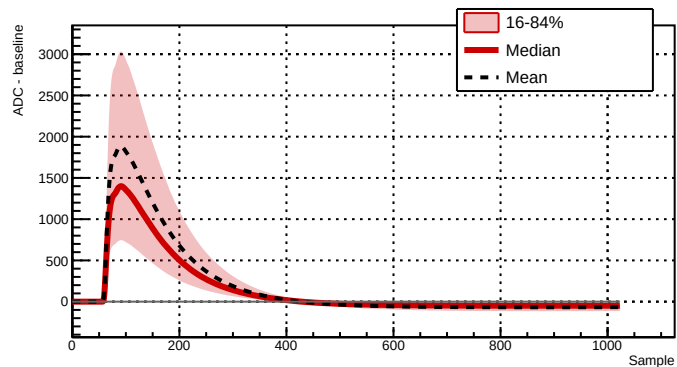
Run 039526 - Channel 2081 - 29081 waveforms
