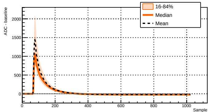
Run 039527 - Channel 2071 - 7834 waveforms
