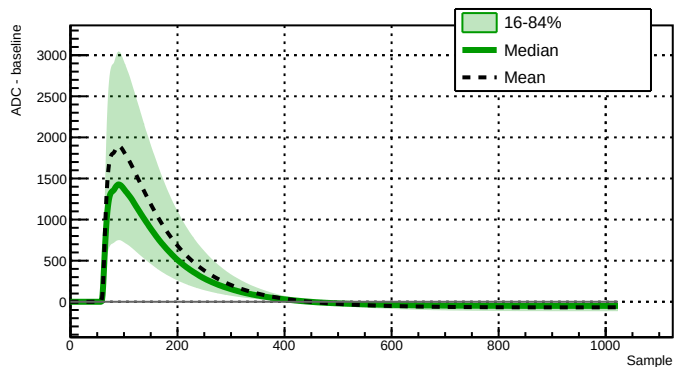
Run 039527 - Channel 2080 - 28903 waveforms
