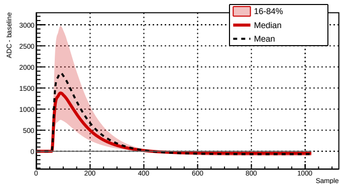
Run 039527 - Channel 2081 - 28657 waveforms
