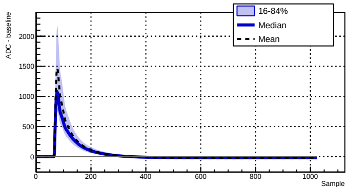
Run 039527 - Channel 2070 - 7894 waveforms
