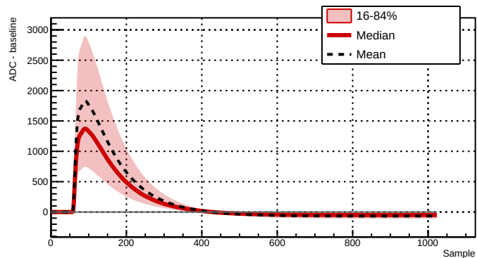
Run 039528 - Channel 2081 - 28276 waveforms
