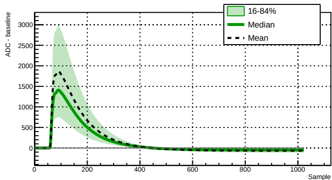
Run 039528 - Channel 2080 - 28605 waveforms
