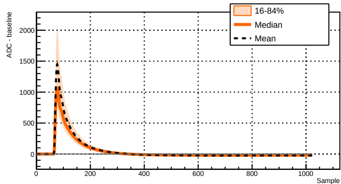
Run 039528 - Channel 2071 - 7725 waveforms
