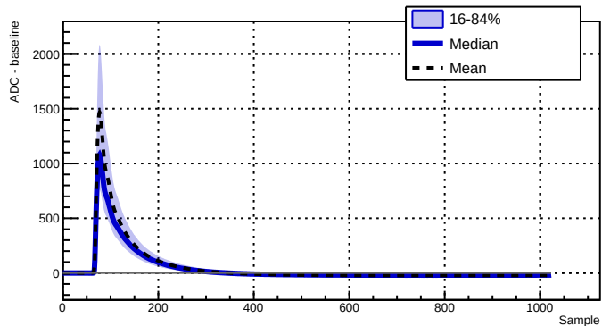
Run 039528 - Channel 2070 - 7869 waveforms
