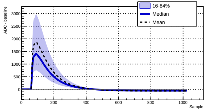
Run 039500 - Channel 2080 - 28366 waveforms
