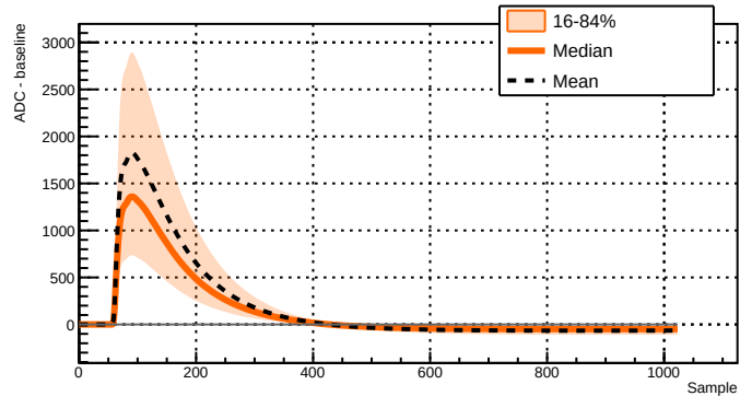
Run 039500 - Channel 2081 - 28202 waveforms
