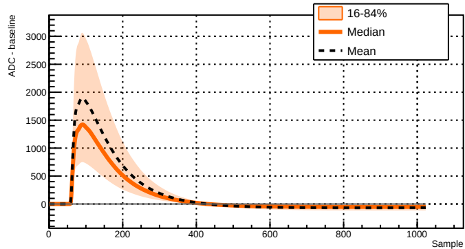
Run 039502 - Channel 2081 - 29964 waveforms
