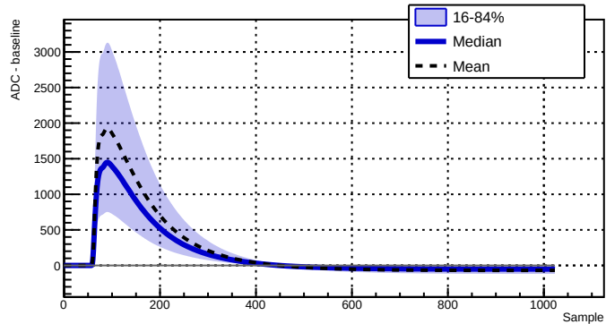
Run 039502 - Channel 2080 - 30346 waveforms
