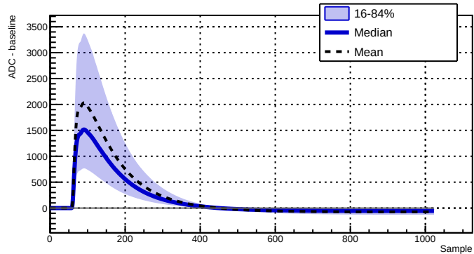
Run 039504 - Channel 2080 - 33156 waveforms
