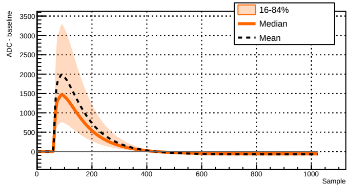
Run 039504 - Channel 2081 - 32997 waveforms
