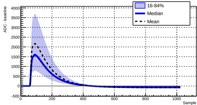
Run 039507 - Channel 2080 - 37503 waveforms
