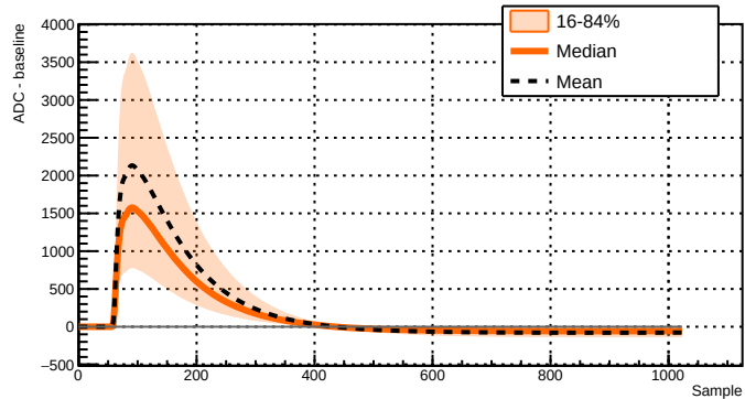
Run 039507 - Channel 2081 - 37143 waveforms
