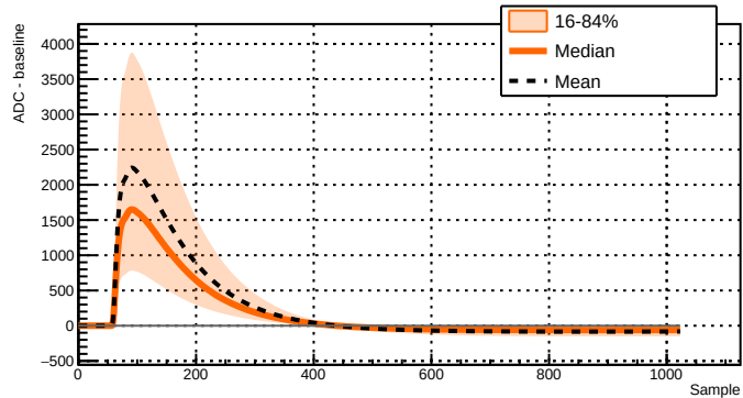
Run 039508 - Channel 2081 - 39014 waveforms
