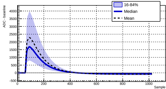
Run 039508 - Channel 2080 - 39128 waveforms
