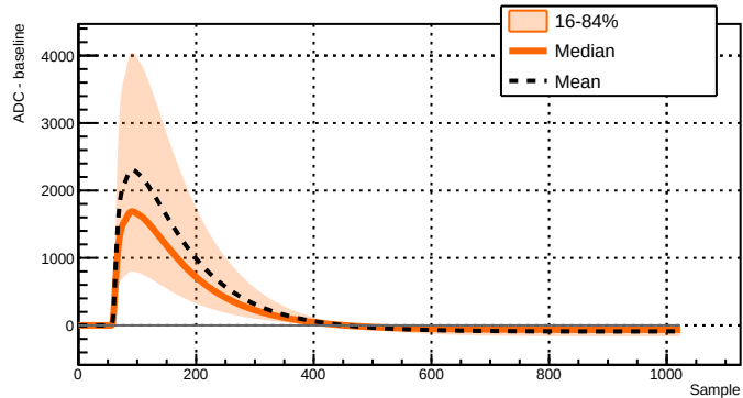
Run 039510 - Channel 2081 - 42029 waveforms
