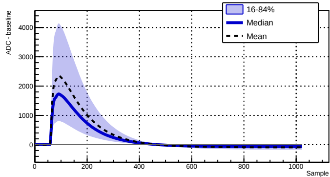
Run 039510 - Channel 2080 - 42194 waveforms
