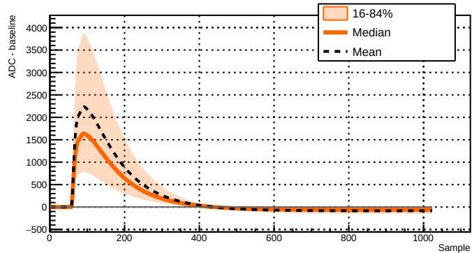
Run 039512 - Channel 2081 - 39305 waveforms
