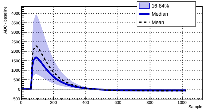
Run 039512 - Channel 2080 - 39399 waveforms
