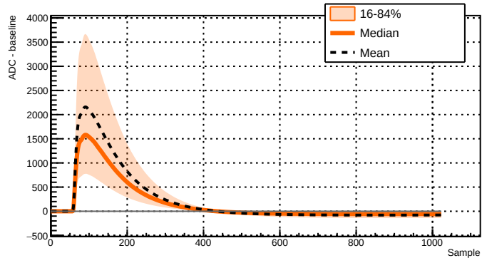
Run 039515 - Channel 2081 - 35671 waveforms
