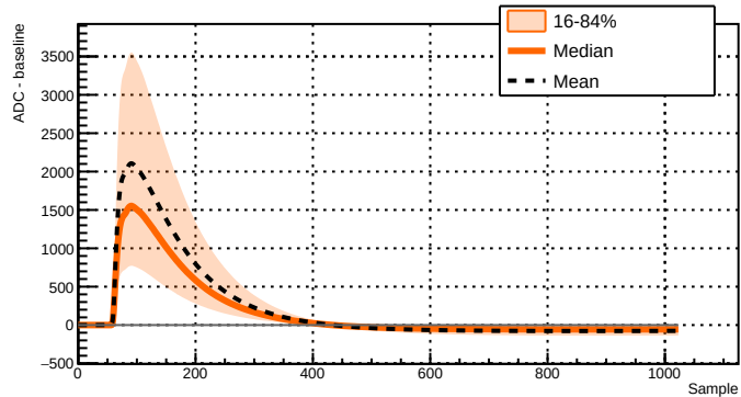
Run 039516 - Channel 2081 - 34599 waveforms
