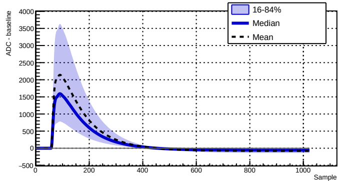
Run 039516 - Channel 2080 - 34859 waveforms
