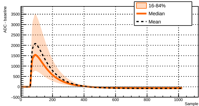
Run 039517 - Channel 2081 - 34553 waveforms
