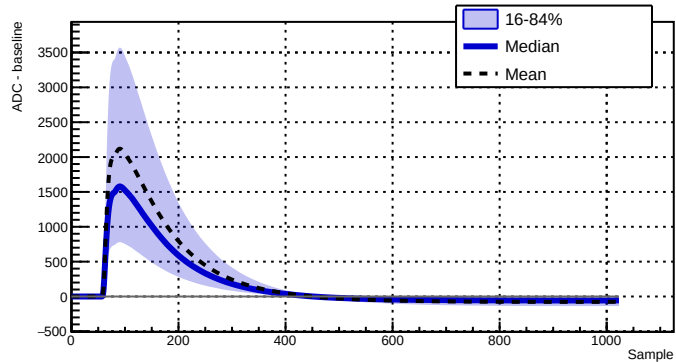
Run 039517 - Channel 2080 - 34628 waveforms
