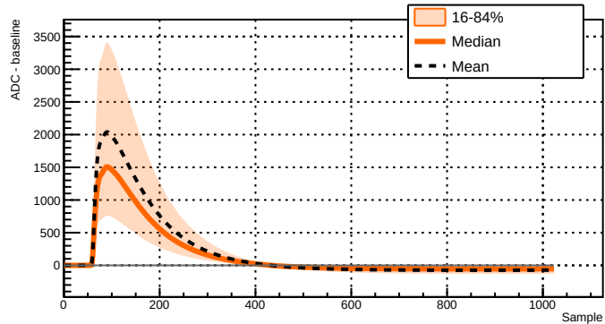
Run 039518 - Channel 2081 - 33784 waveforms
