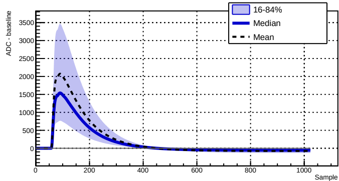
Run 039518 - Channel 2080 - 33905 waveforms
