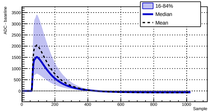
Run 039519 - Channel 2080 - 33043 waveforms
