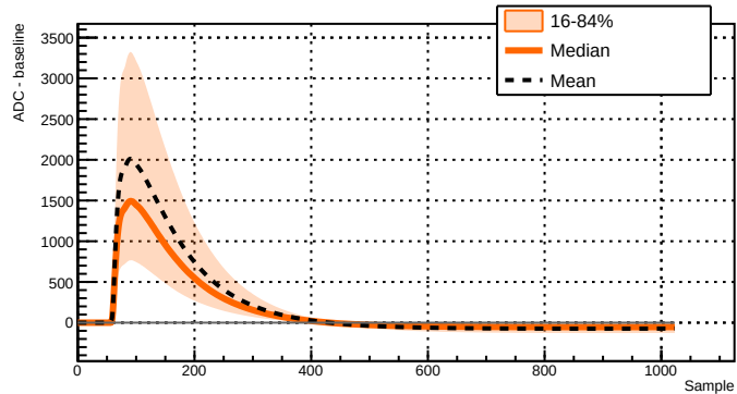
Run 039519 - Channel 2081 - 32744 waveforms
