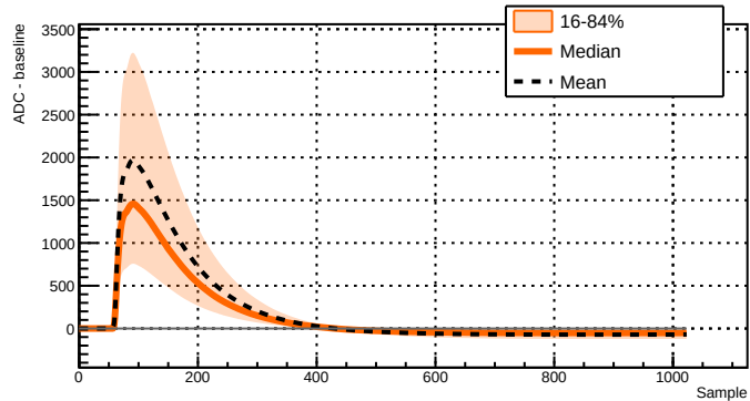
Run 039521 - Channel 2081 - 31524 waveforms
