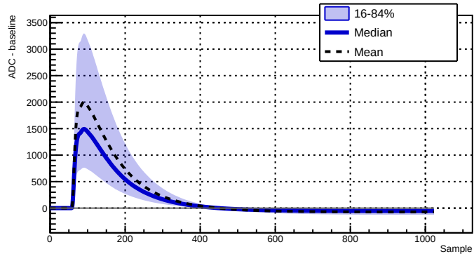
Run 039521 - Channel 2080 - 31828 waveforms
