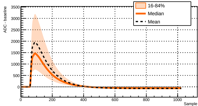
Run 039522 - Channel 2081 - 31313 waveforms
