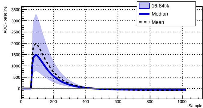
Run 039522 - Channel 2080 - 31446 waveforms
