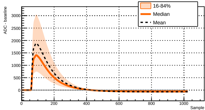
Run 039525 - Channel 2081 - 29317 waveforms
