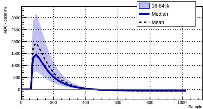
Run 039525 - Channel 2080 - 29606 waveforms
