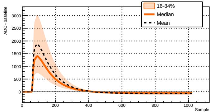
Run 039526 - Channel 2081 - 29118 waveforms
