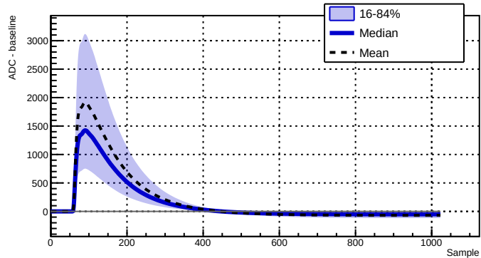
Run 039526 - Channel 2080 - 29374 waveforms
