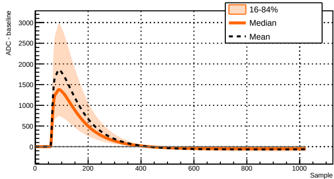
Run 039527 - Channel 2081 - 28667 waveforms
