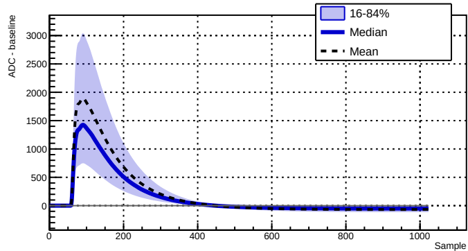
Run 039527 - Channel 2080 - 28971 waveforms
