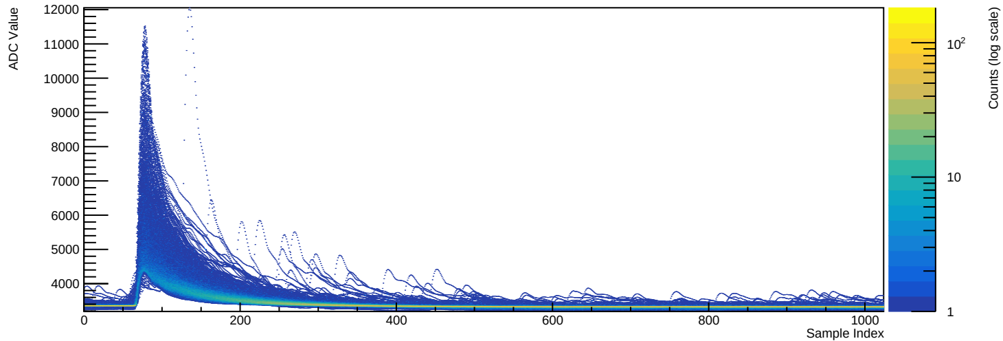
Run 039512 - Channel 2070 (n=2764 waveforms)
