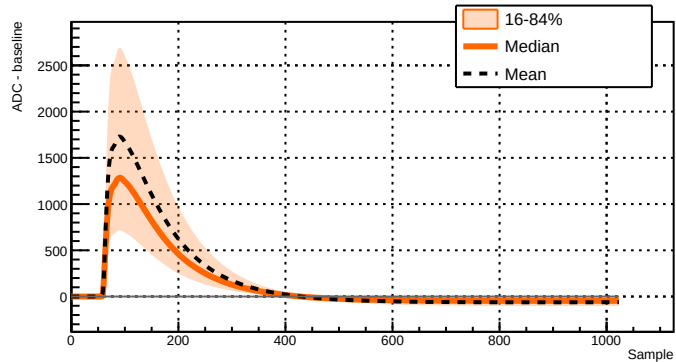
Run 039500 - Channel 2081 - 22792 waveforms
