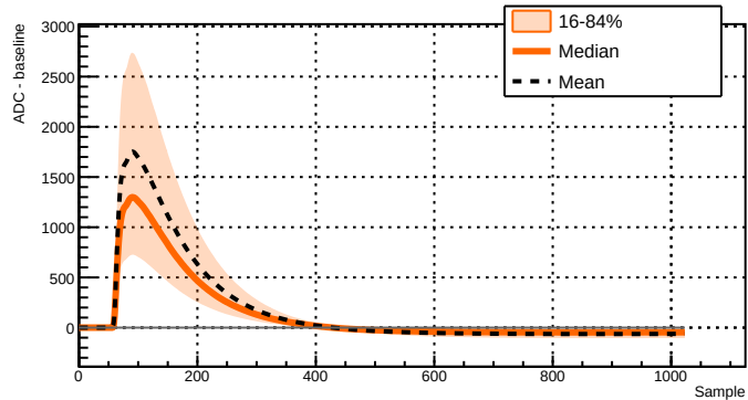
Run 039501 - Channel 2081 - 23475 waveforms
