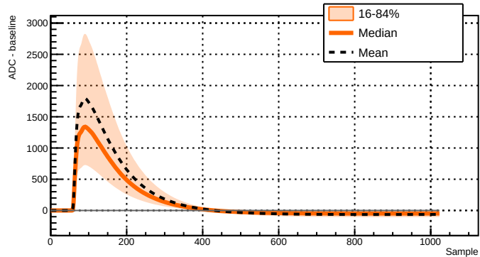
Run 039502 - Channel 2081 - 24509 waveforms
