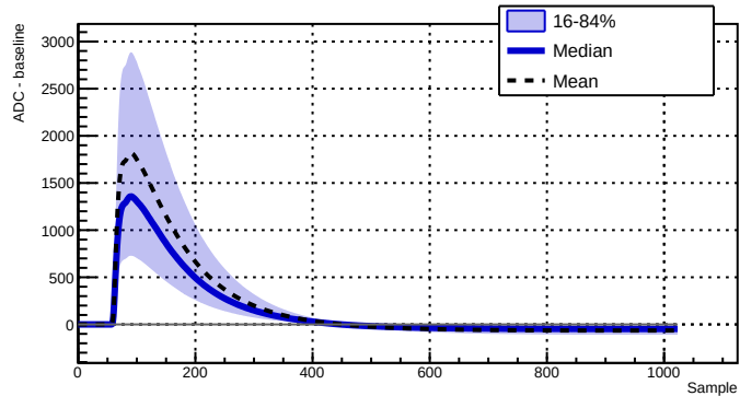
Run 039502 - Channel 2080 - 25032 waveforms
