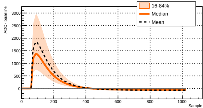
Run 039503 - Channel 2081 - 25682 waveforms
