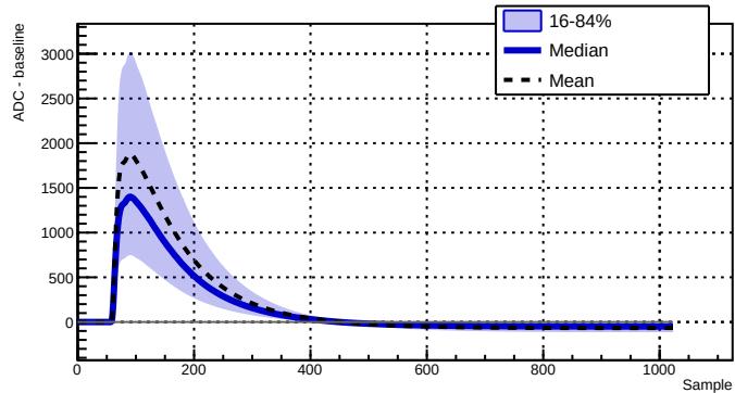
Run 039503 - Channel 2080 - 26220 waveforms
