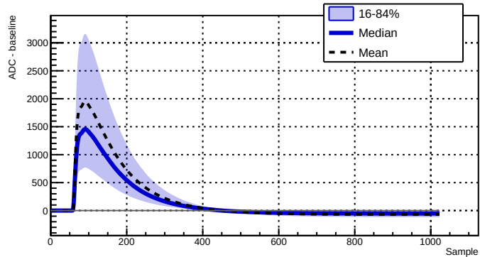
Run 039504 - Channel 2080 - 26974 waveforms
