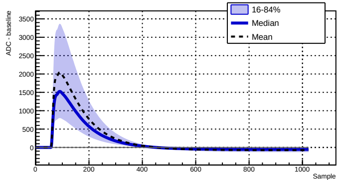
Run 039506 - Channel 2080 - 28277 waveforms
