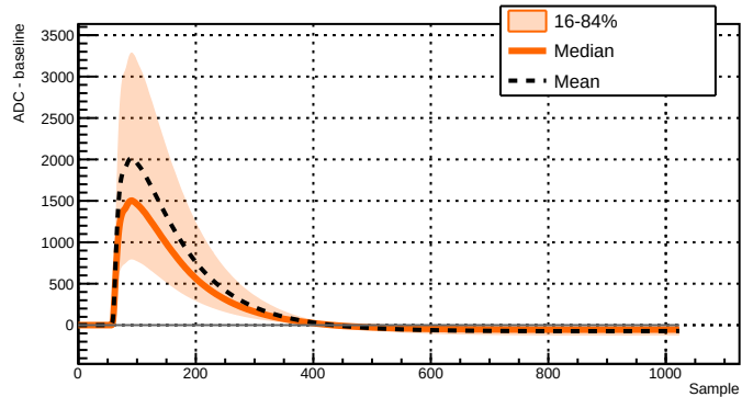
Run 039506 - Channel 2081 - 27864 waveforms
