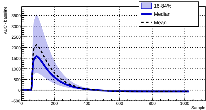
Run 039507 - Channel 2080 - 30015 waveforms
