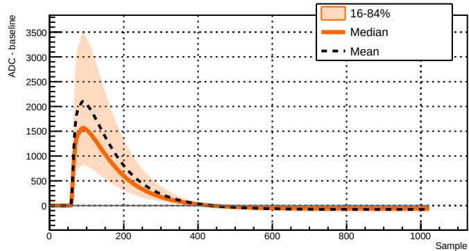
Run 039507 - Channel 2081 - 29486 waveforms
