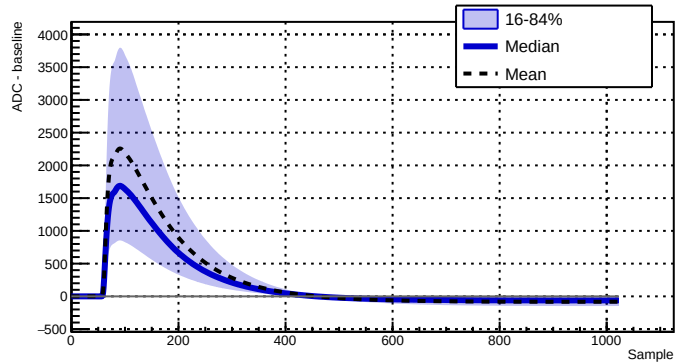
Run 039508 - Channel 2080 - 30930 waveforms
