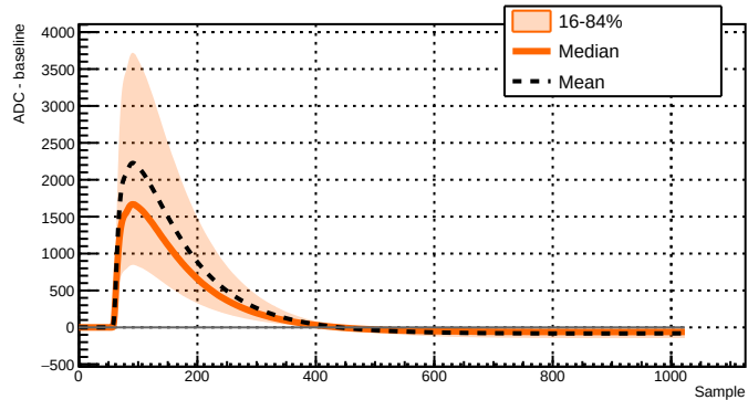
Run 039508 - Channel 2081 - 30558 waveforms
